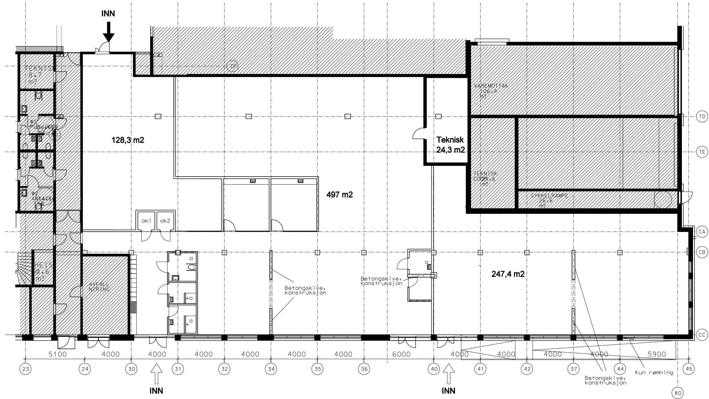
PLANLAYOUT 1:200
